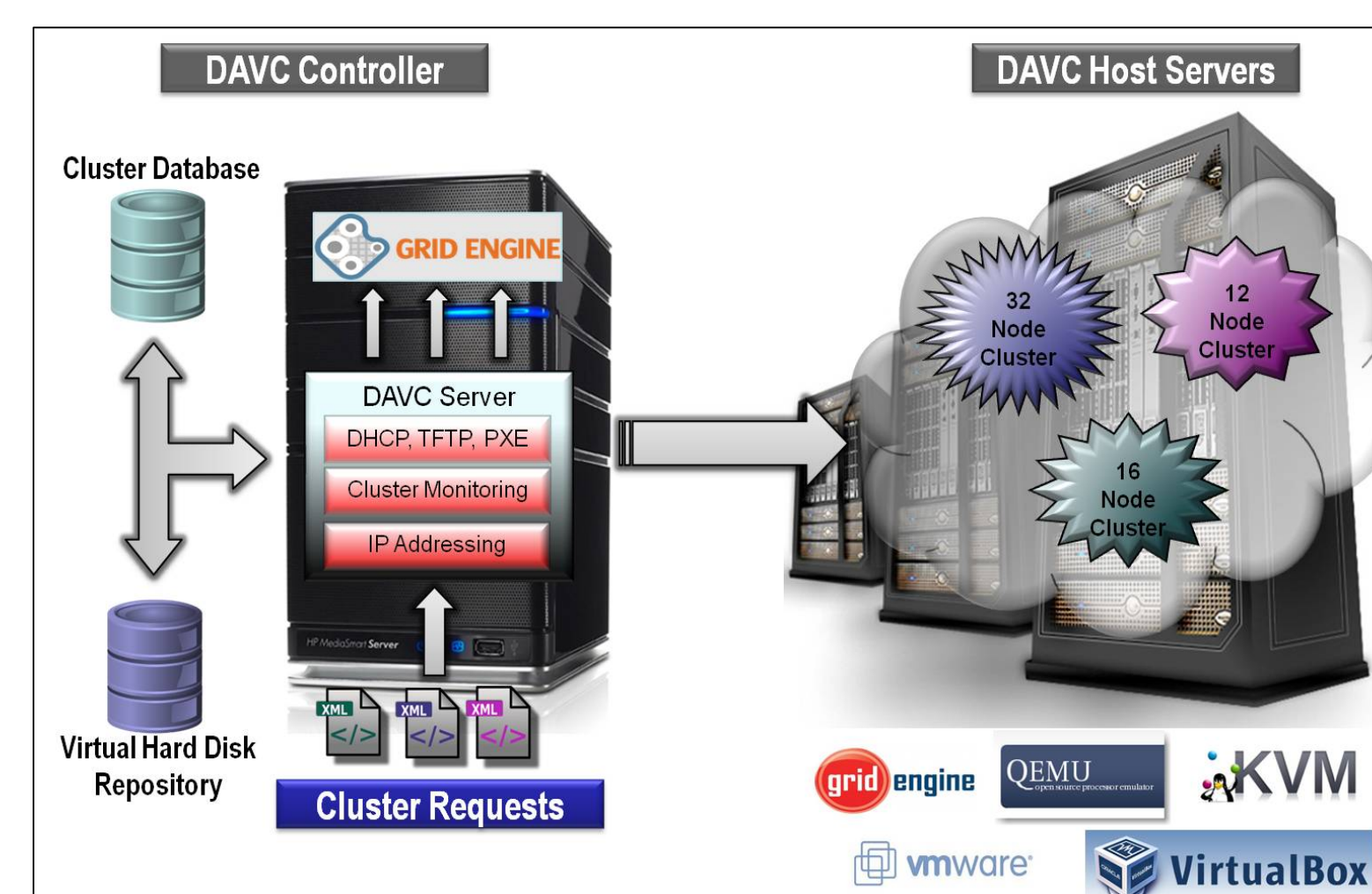
Dynamically Allocated Virtual Clusters (DAVC)
