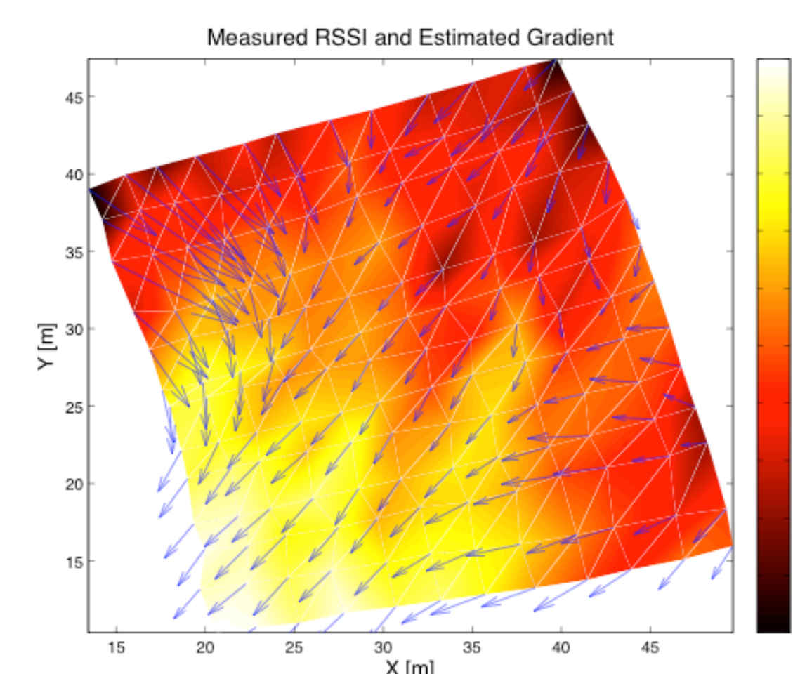
Track RSS Gradient to inform mobility decisions
