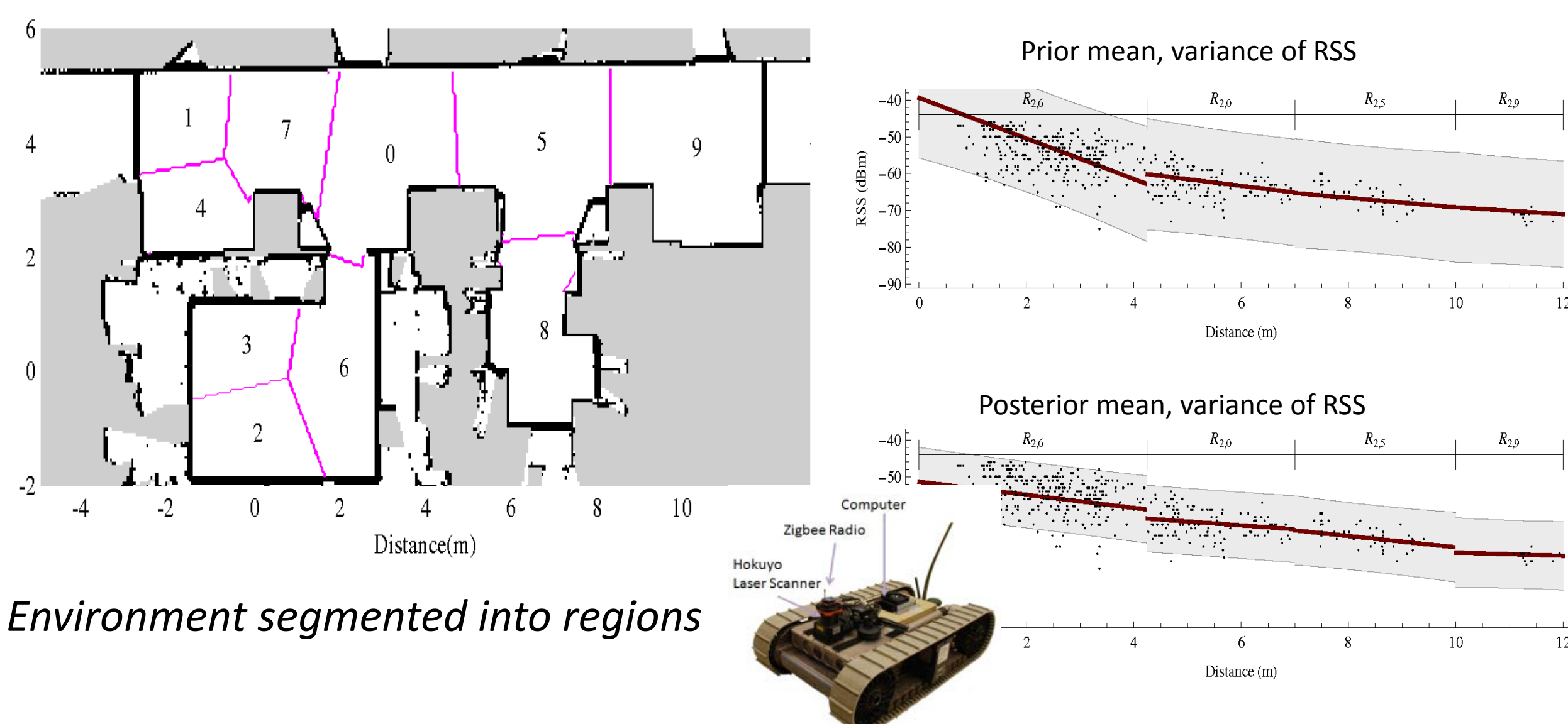
Online learning of mobile-to-mobile channel
