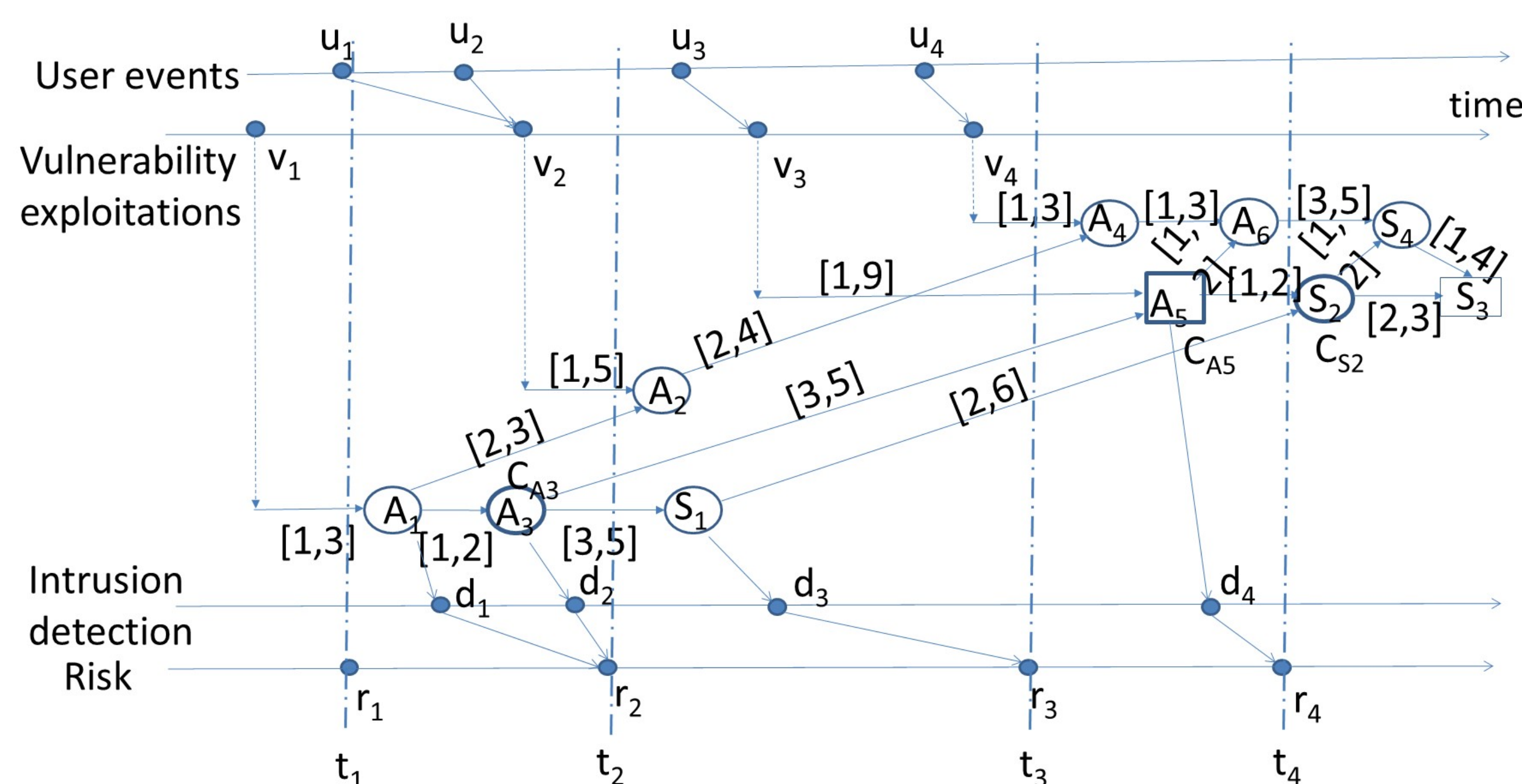
Controlling influence of vulnerability exploitation on assets and services
