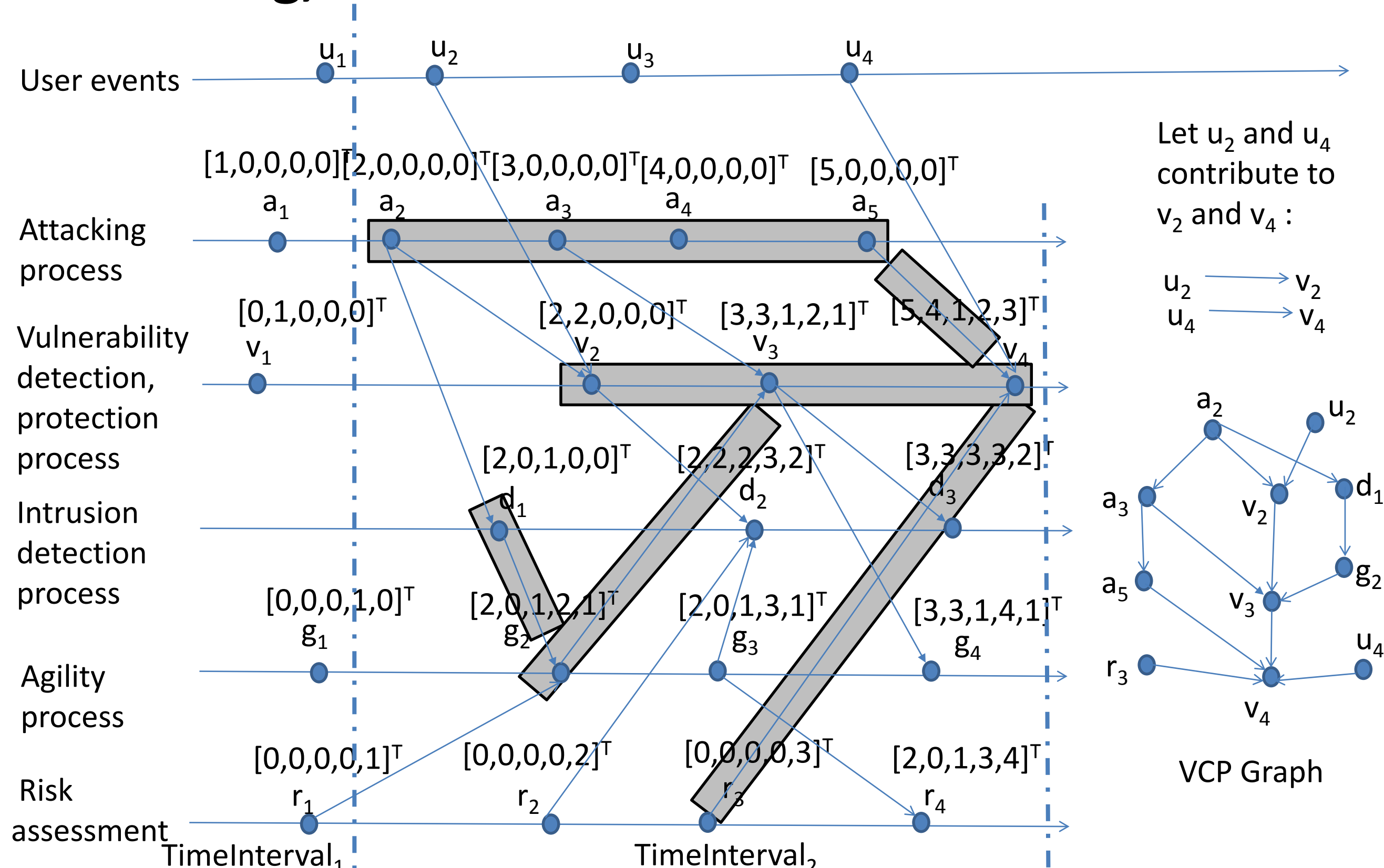
Temporal causal history of cyber and user events with vulnerability-centric pairing graph
