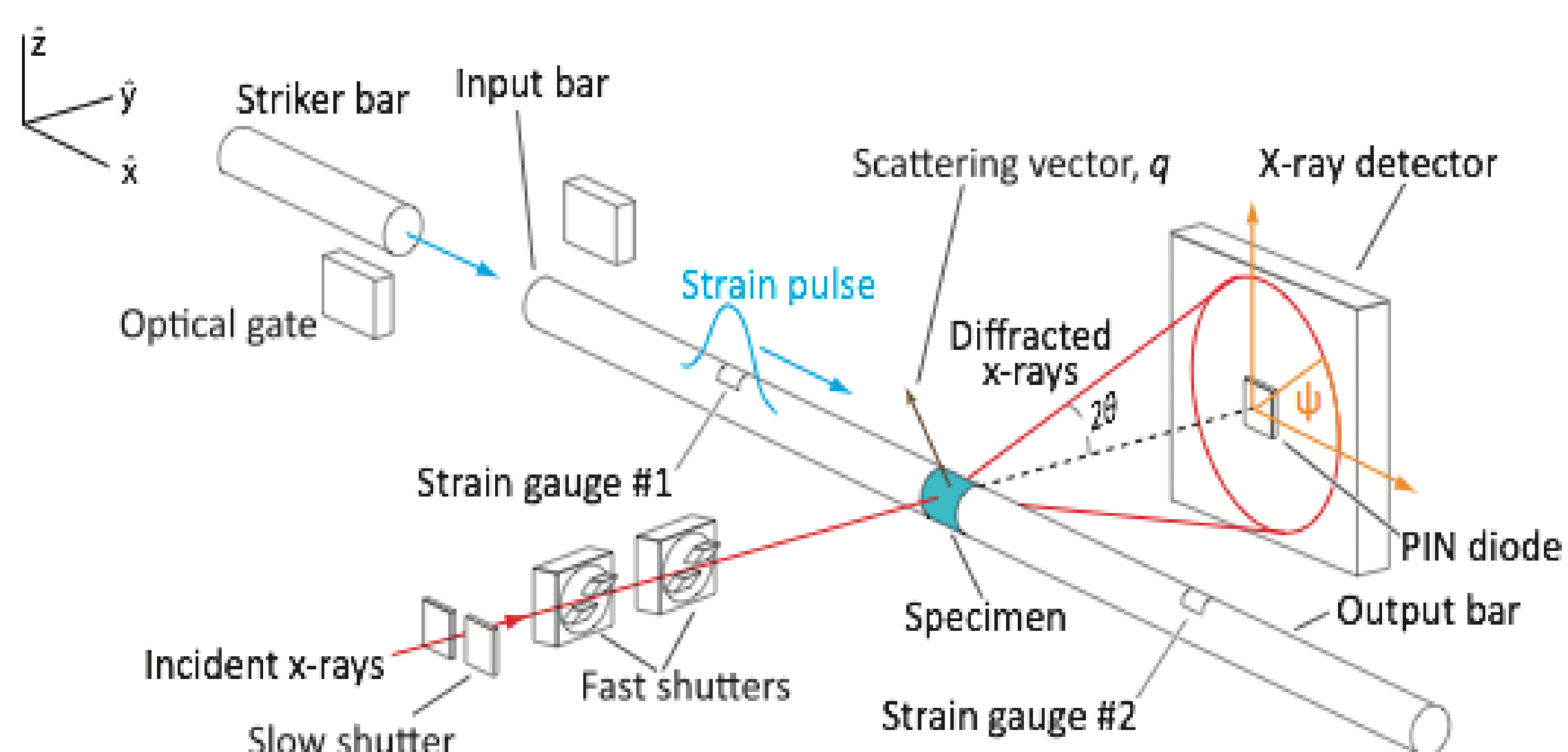
A Kolsky bar configured for in situ XRD.
